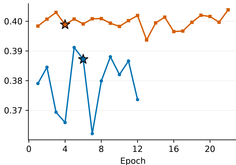
Clustering MMD ratio \downarrow
