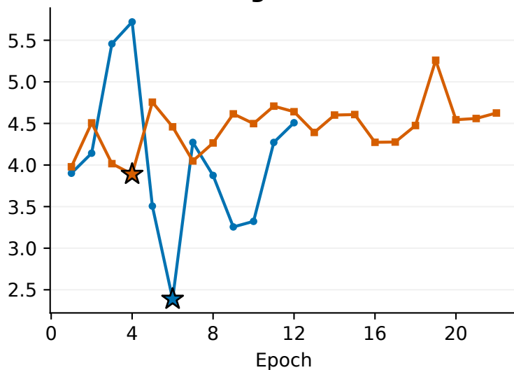
Clustering MMD ratio \downarrow
