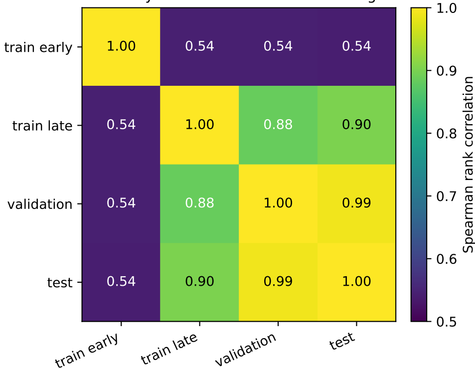
Stability of learned interaction rankings
