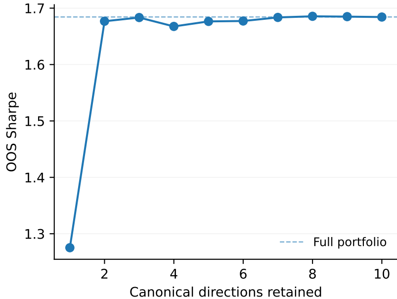
Economic value under truncation
