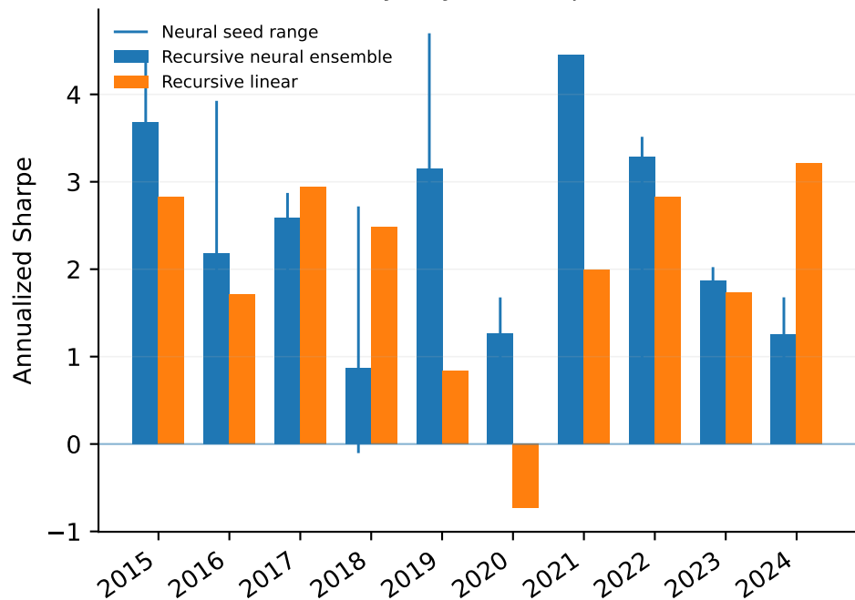
Payoff-year Sharpe
