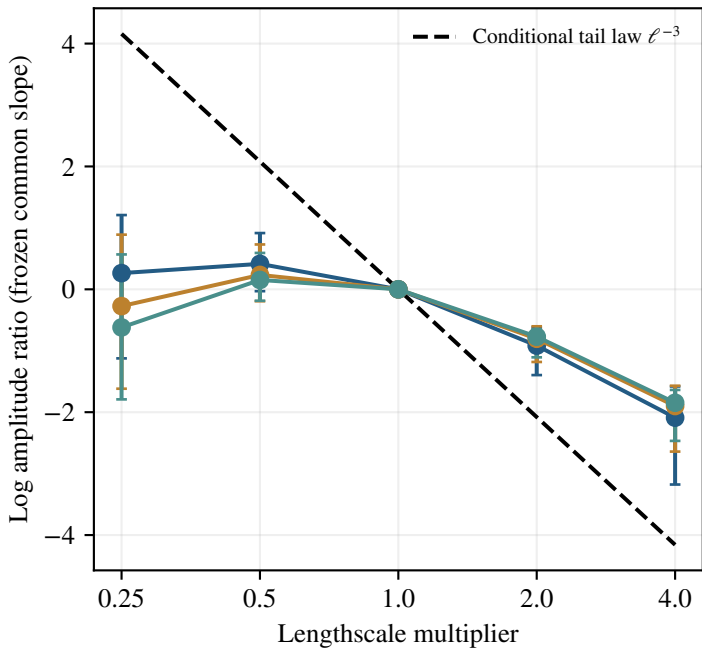
Finite-range proxy versus conditional tail law
