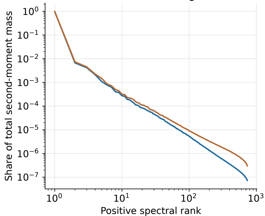
Mass-normalized diagnostic
