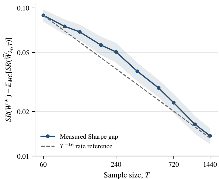
(b) Sharpe learning rate
