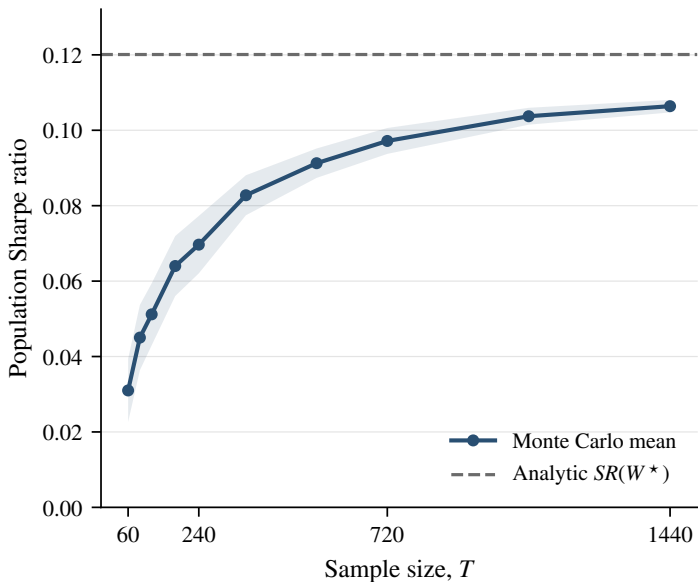
(a) Sharpe ratio recovery
