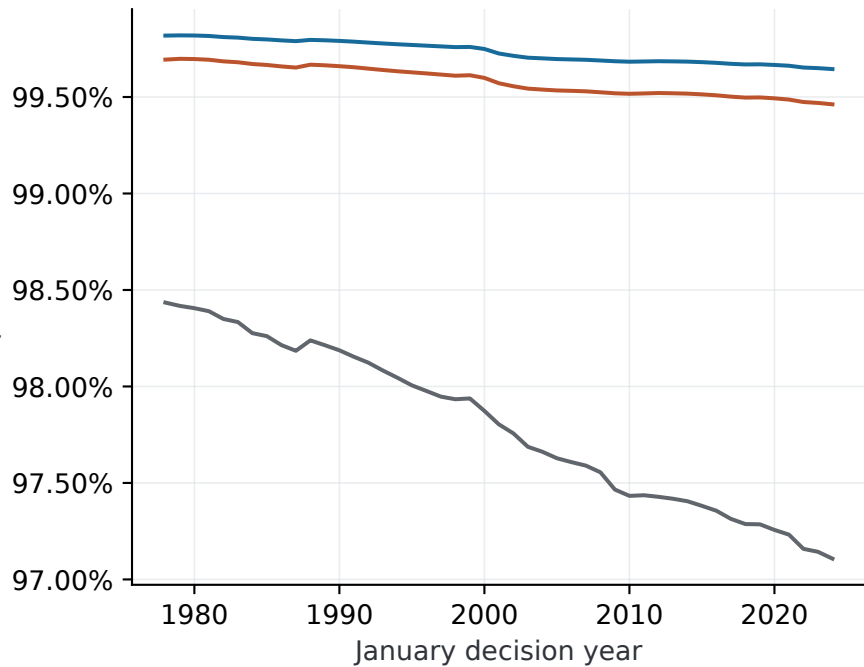
Eigenvalue mass share in the top 10 directions
