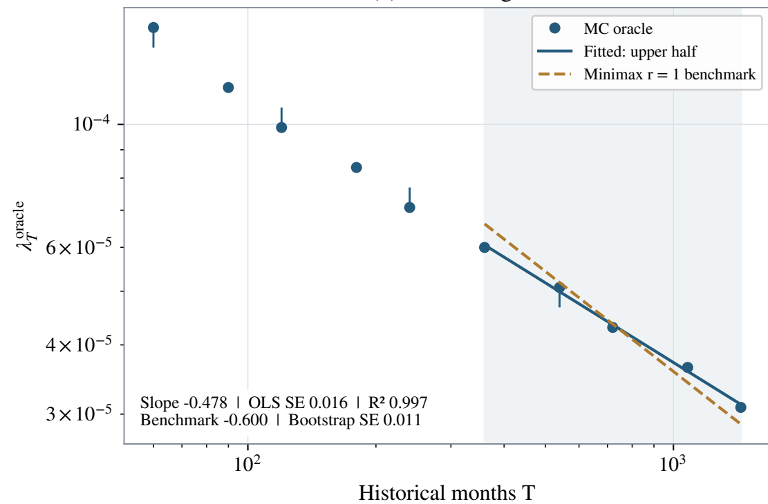
(b) Oracle ridge
