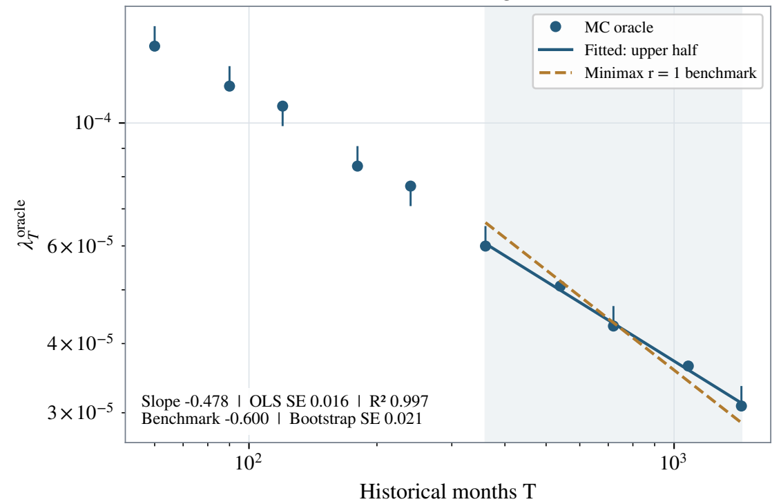
(b) Oracle ridge
