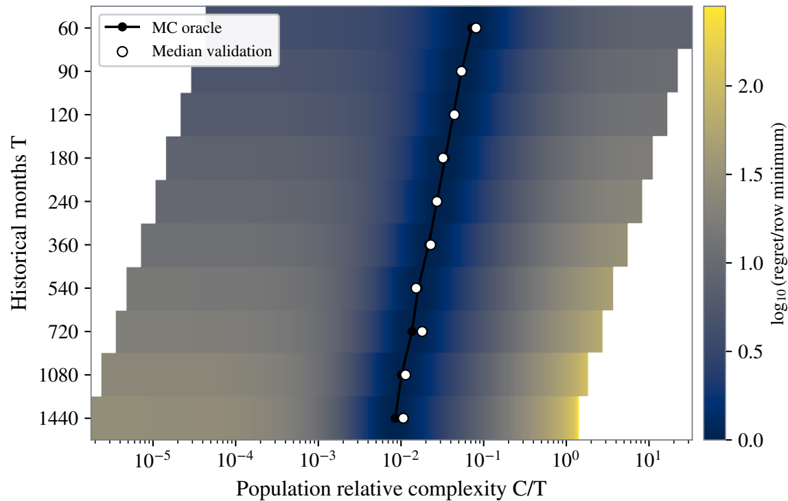
(a) Finite-sample learnability map
