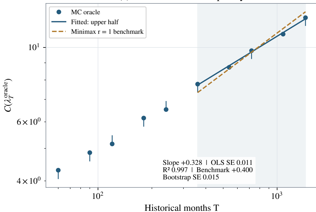
(c) Oracle effective complexity
