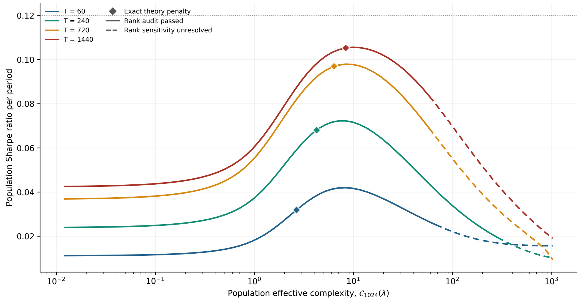
Figure 3. Sharpe versus effective complexity
