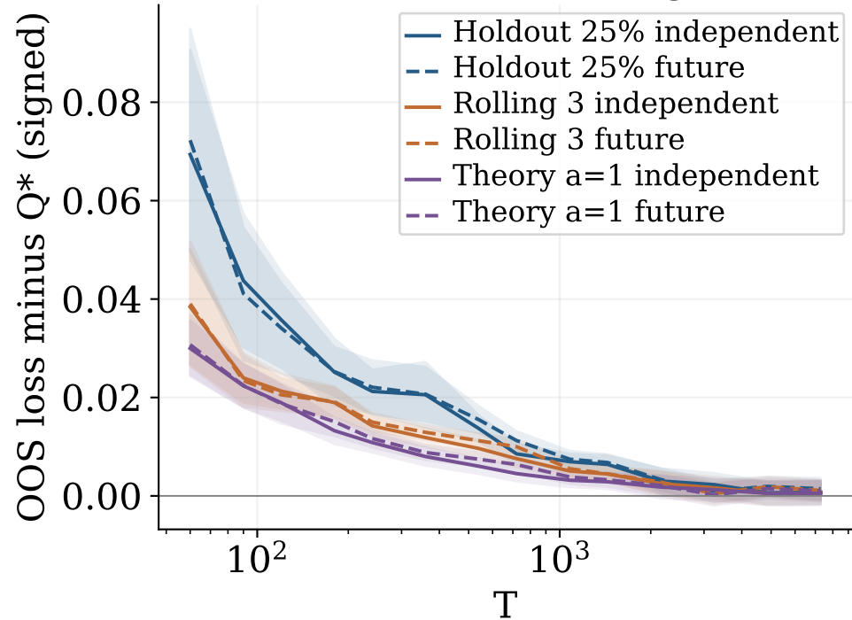
Independent versus contiguous OOS
