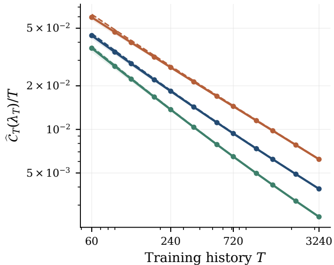
(b) Relative empirical complexity
