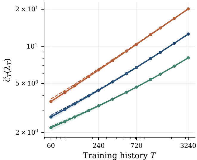
(a) Empirical effective complexity
