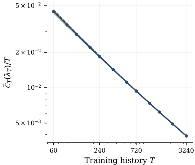
(b) Relative empirical complexity
