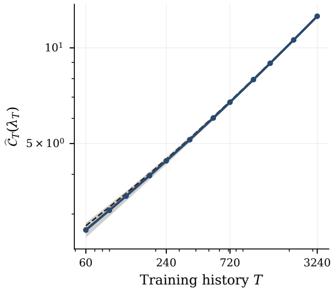
(a) Empirical effective complexity
