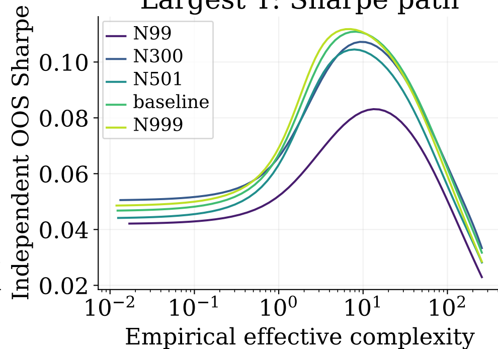
Largest T: Sharpe path
