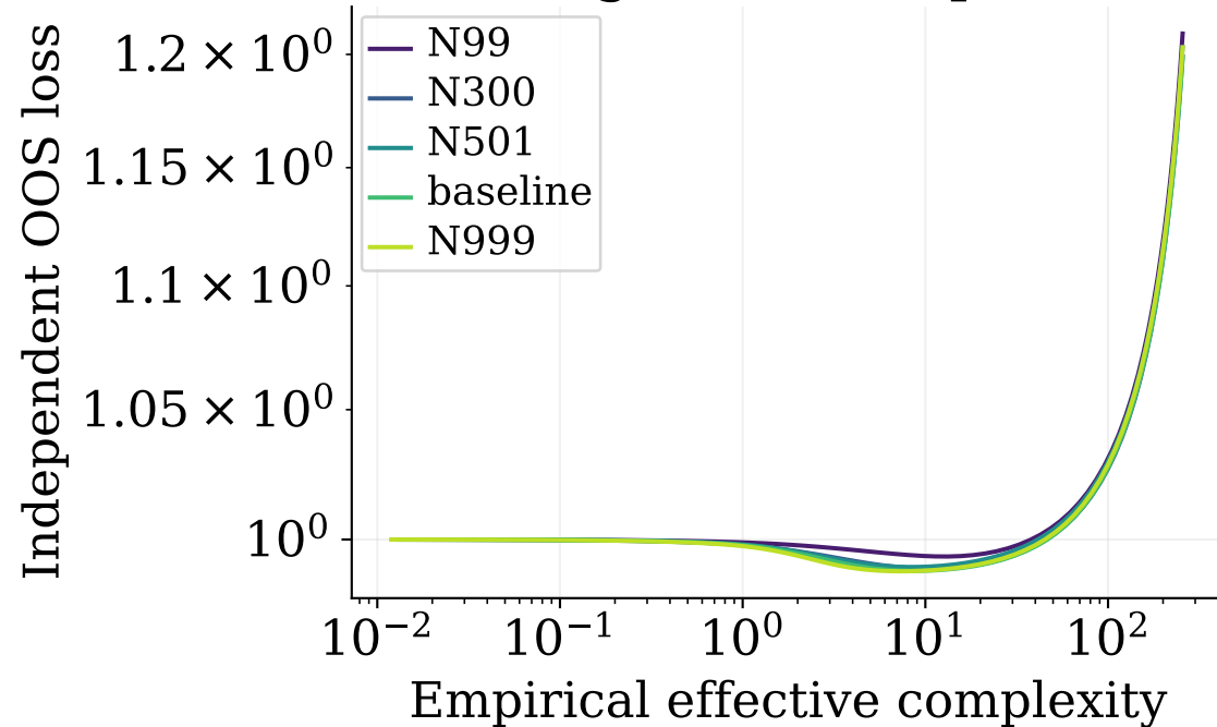
Largest T: loss path
