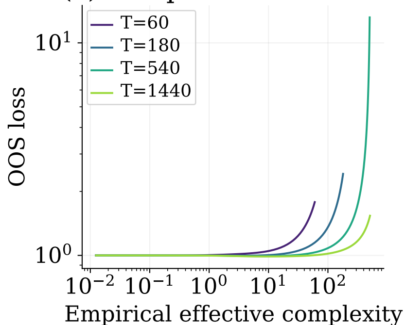
(c) OOS loss by T
