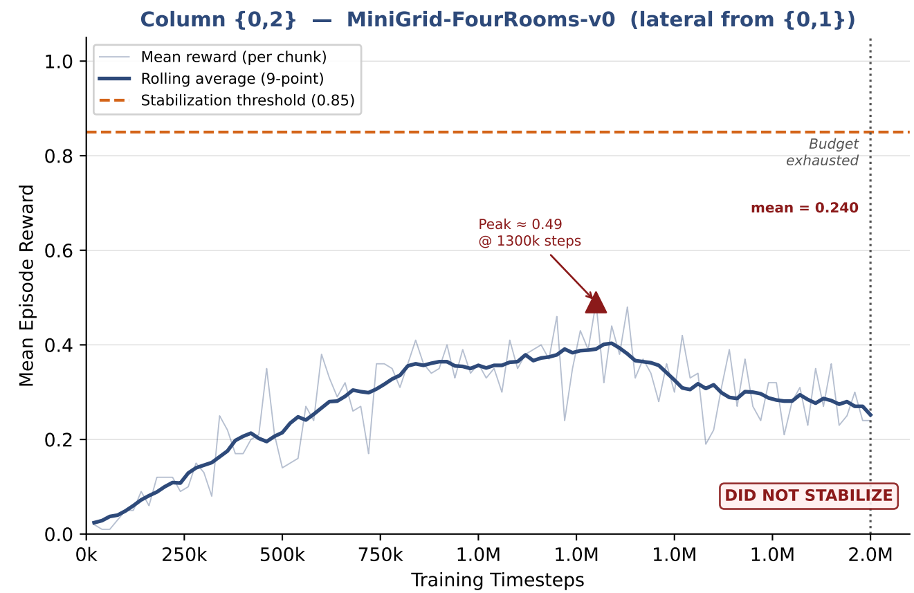
Figure 2 — PN-4 Training Curves: Progressive Network Column Training
