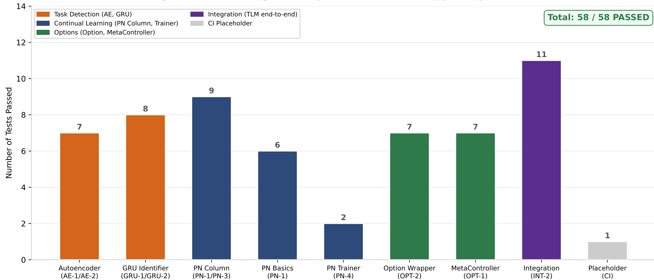
Figure 5 — Test Coverage Summary: 58 / 58 Tests Passed (pytest, Python 3.10)
