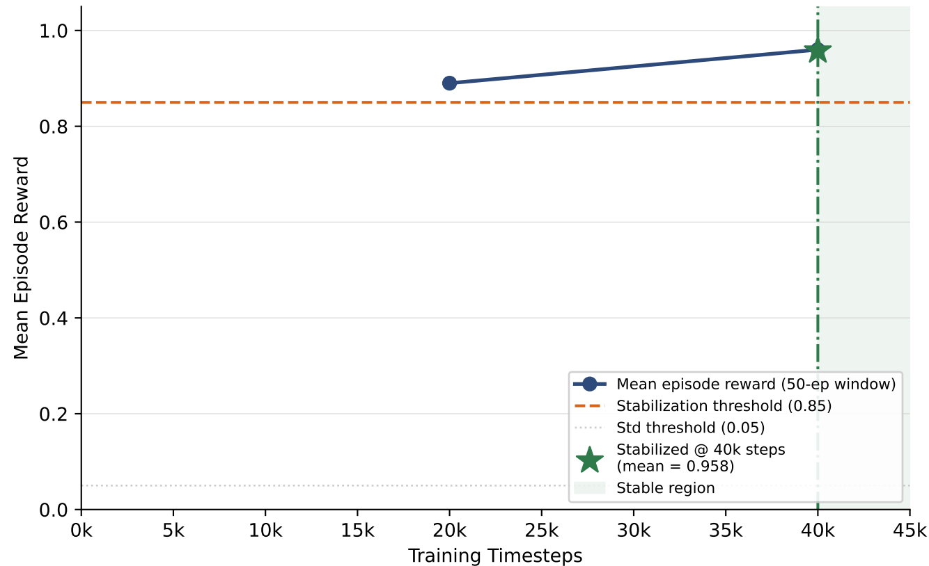
Column {0,1} — MiniGrid-Empty-8x8-v0
