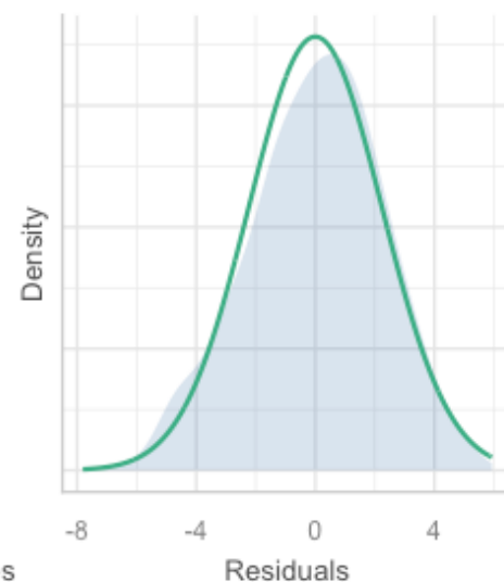
Normality of Residuals Distribution should be close to the normal
