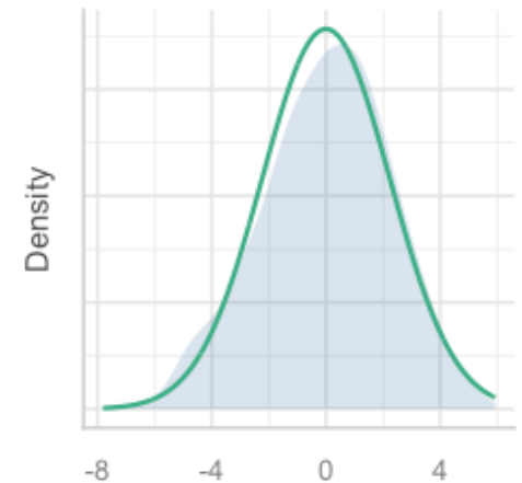
Normality of Residuals
