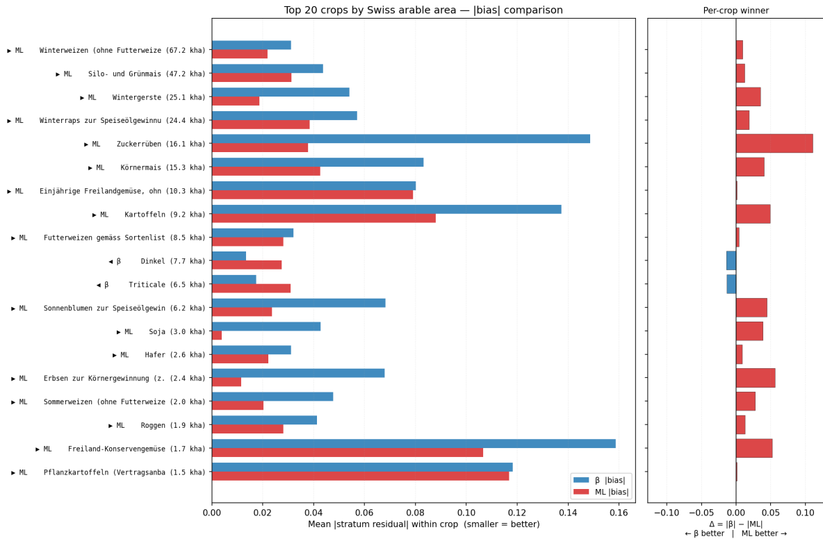
Figure 5: Comparison of ML and calibrated function approach for the top 20 crops (per area).
