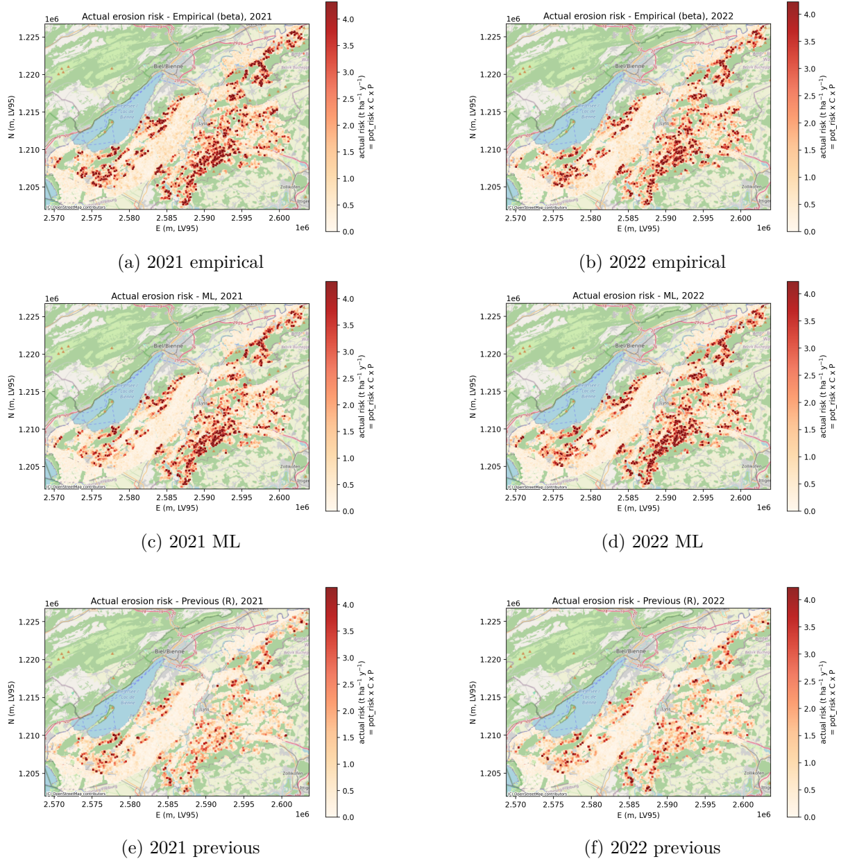
Figure 22: Actual erosion risk [ \text{t ha}^{-1} \text{y}^{-1} ] in 2021 and 2022, using C-factors from the empirical model, ML model and previous results. On value is shown per field at it's centroid.
