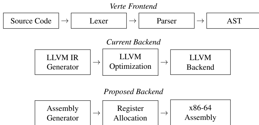
Figure 1: Verte Compiler architecture, showing existing and proposed backends.
