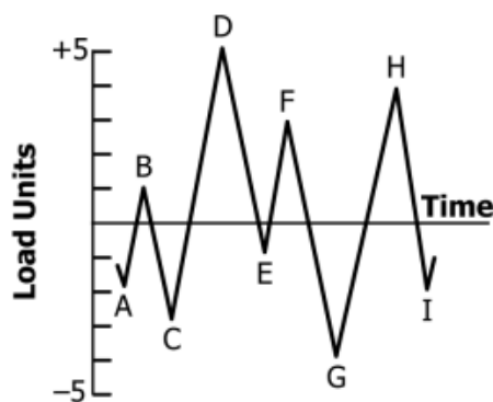
Original load history
