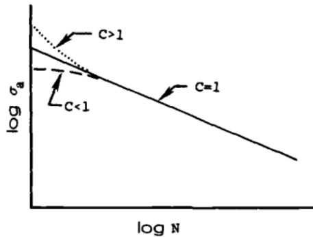
Figure 3 : Effect of parameter C on the S-N curve
