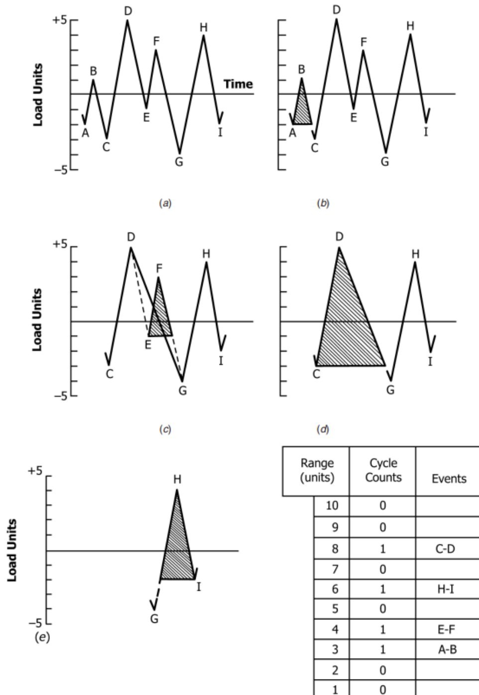
FIG. 5 Range-Pair Counting Example
