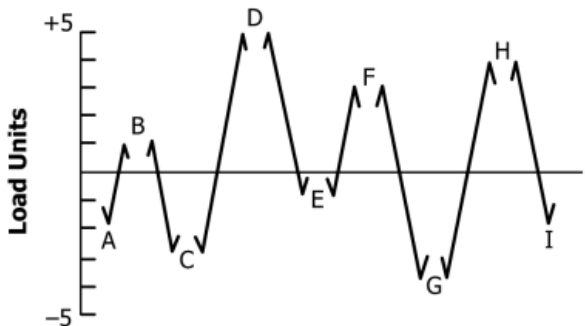
FIG. 4 Simple Range Counting Example—Both Positive and Negative Ranges Counted
