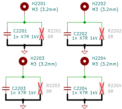
Drilling Holes
