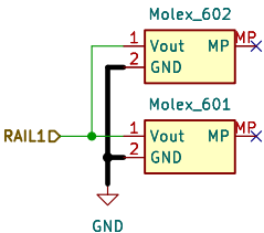
Output Rail 1
