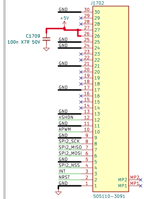
External Connector
