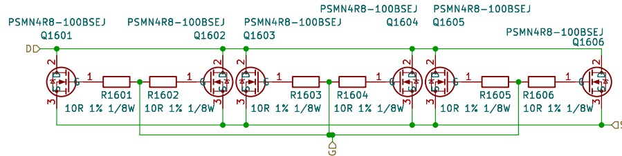
Power Hot-Swap Circuit
