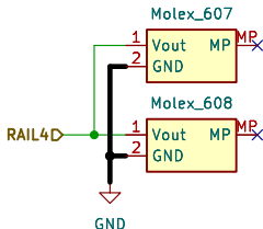
Output Rail 4
