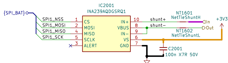
Batterie Voltage, Current and Temperature Sensor
