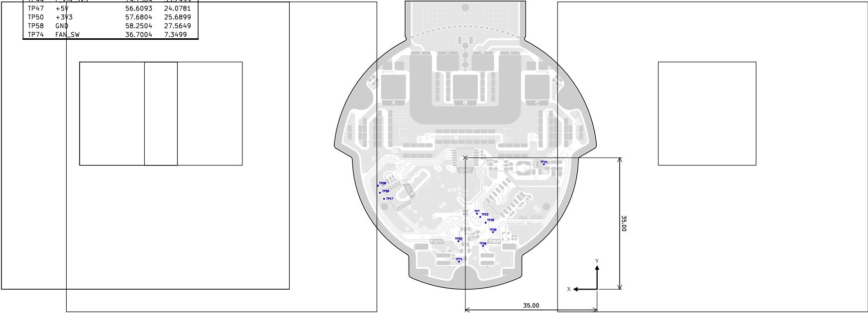
Bottom Test Points (Scale 1:1)
