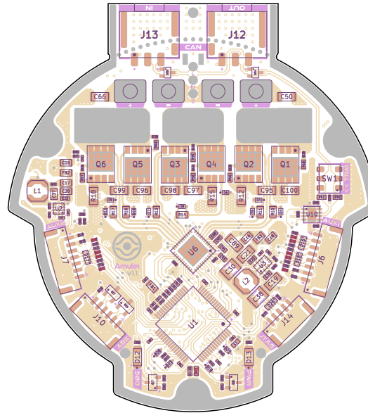
Top Assembly (scale 1:1)
