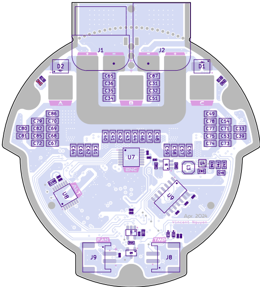
Bottom Assembly (scale 1:1)
