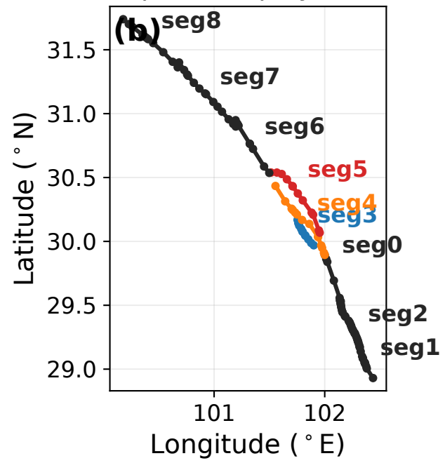
Fault trace, map view (splay strands coloured)
