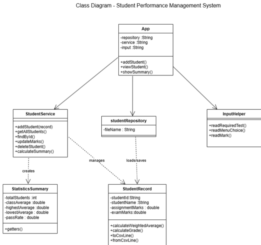
Figure 2: Class Diagram
