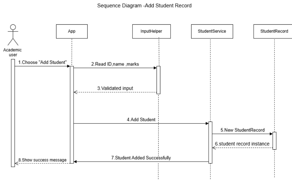
Figure 4: Sequence Diagram
