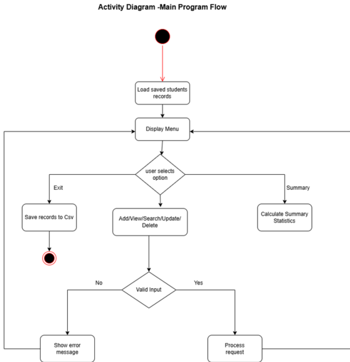
Figure 3: Activity Diagram
