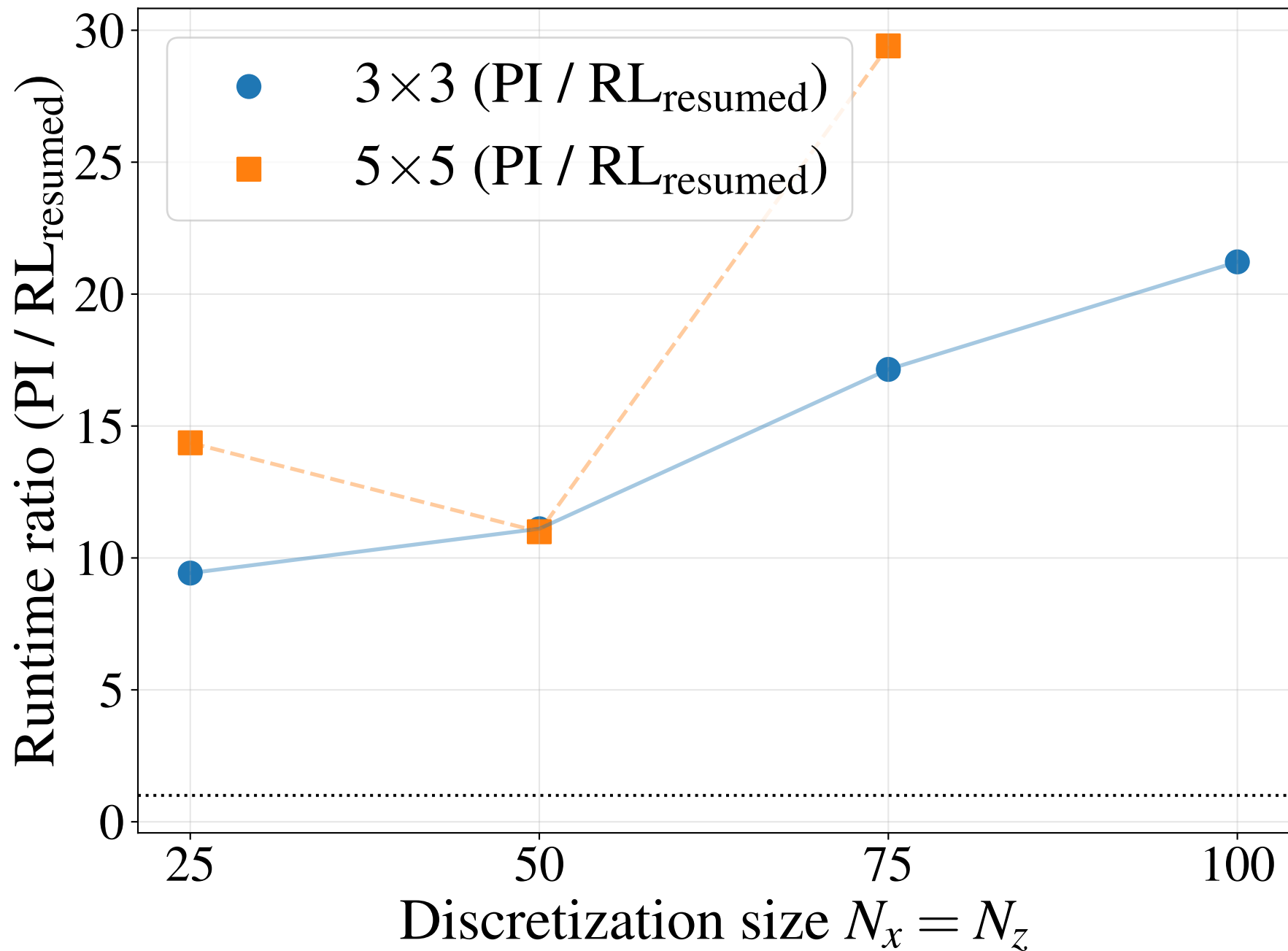
PI vs RESUMED RL: runtime ratio vs discretization
