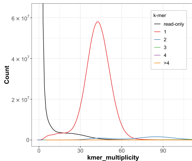
Distribution of k-mer counts per copy numbers found in assembly_01 (hapl.)
