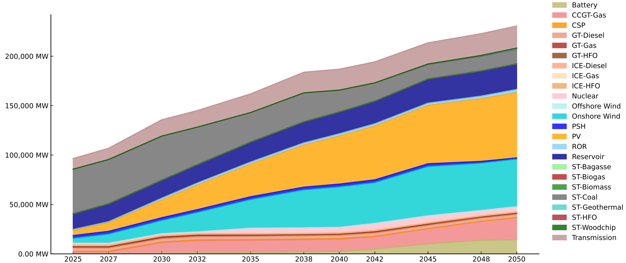
Installed Capacity System - baseline [MW]
