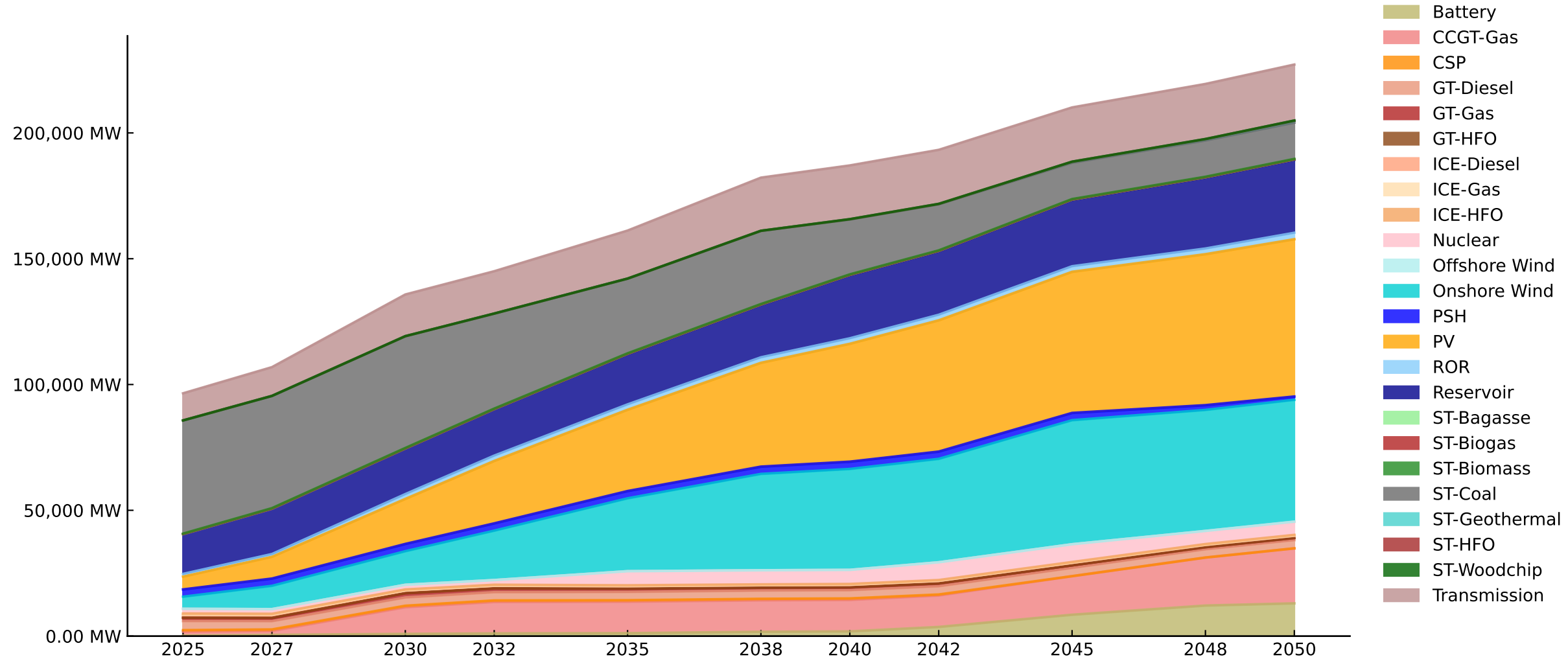
Installed Capacity System - baseline_INGA [MW]
