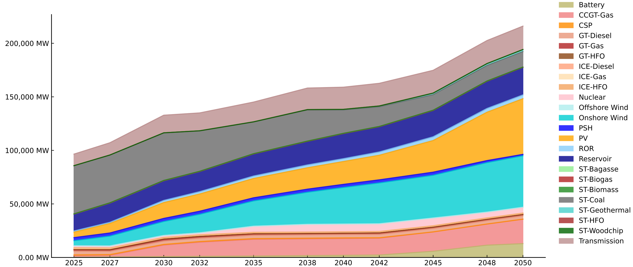
Installed Capacity System - baseline_limexp [MW]
