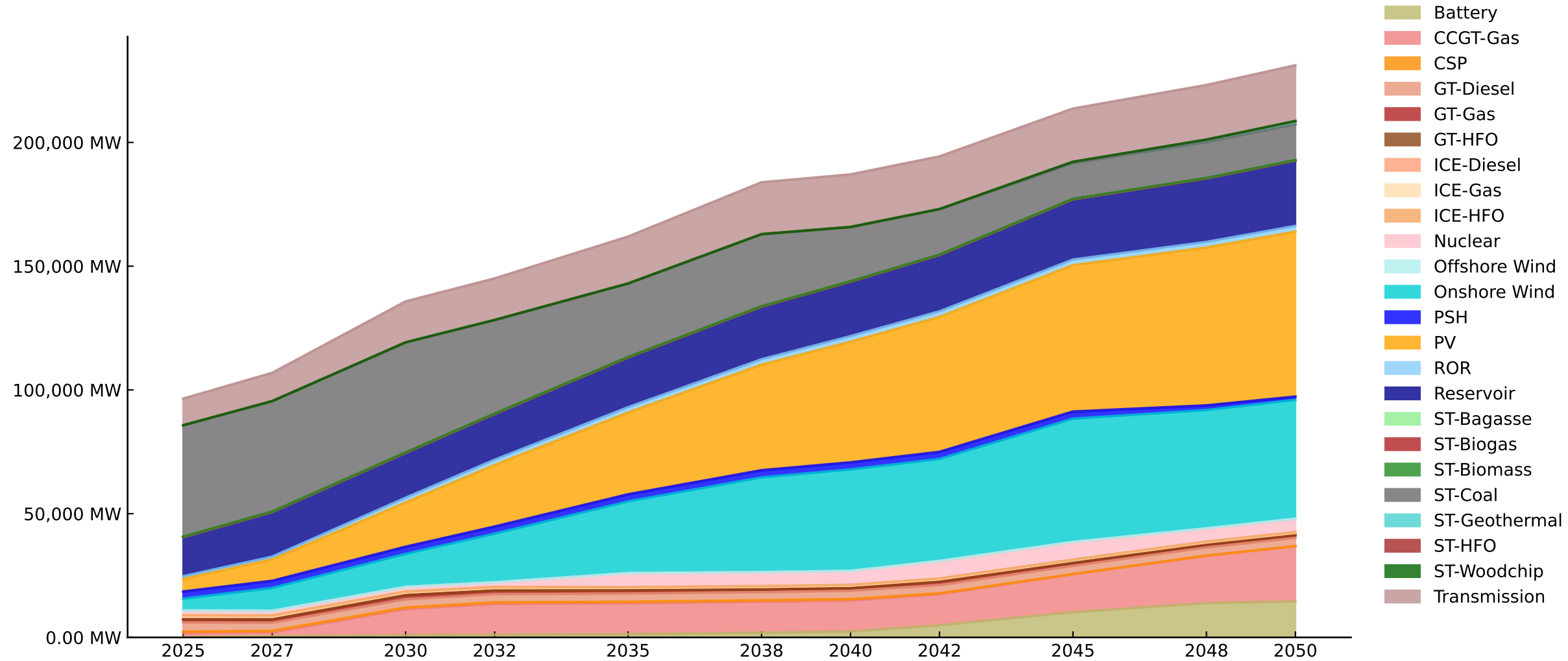
Installed Capacity System - baseline_noBTKG [MW]
