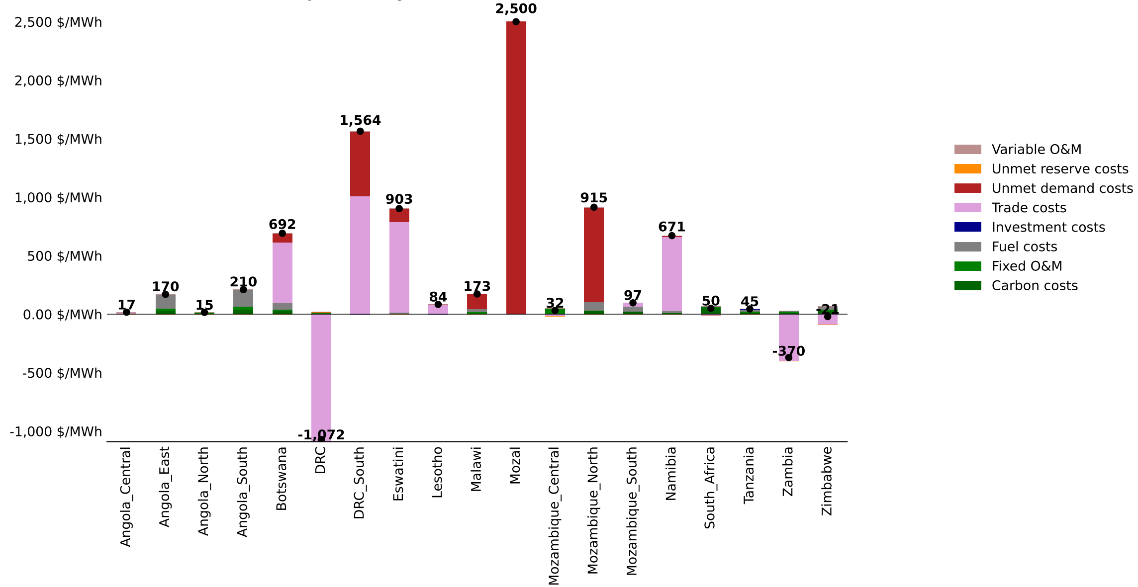
Cost Composition by Zone in 2025 - baseline (USD/MWh)
