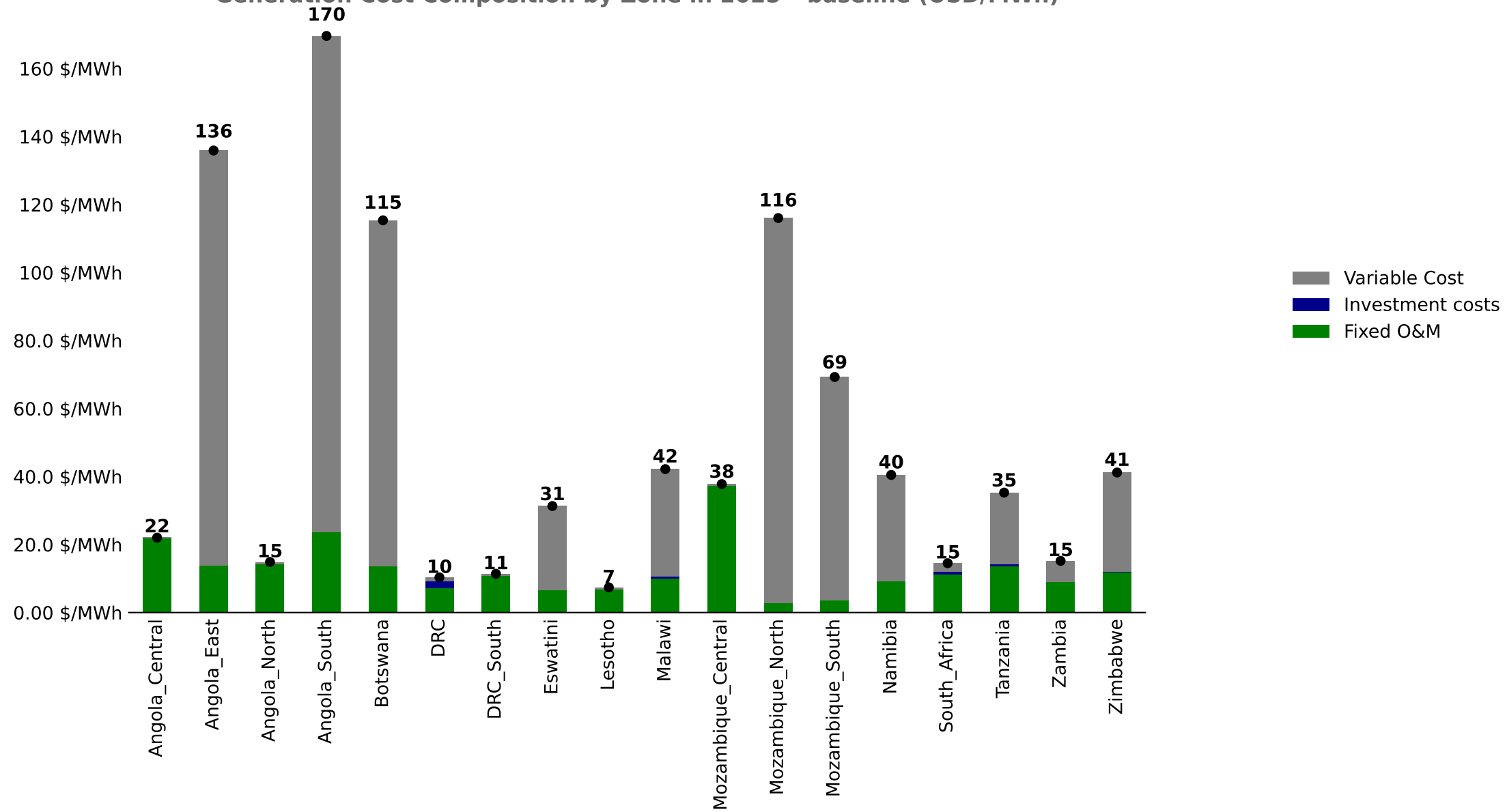
Generation Cost Composition by Zone in 2025 - baseline (USD/MWh)
