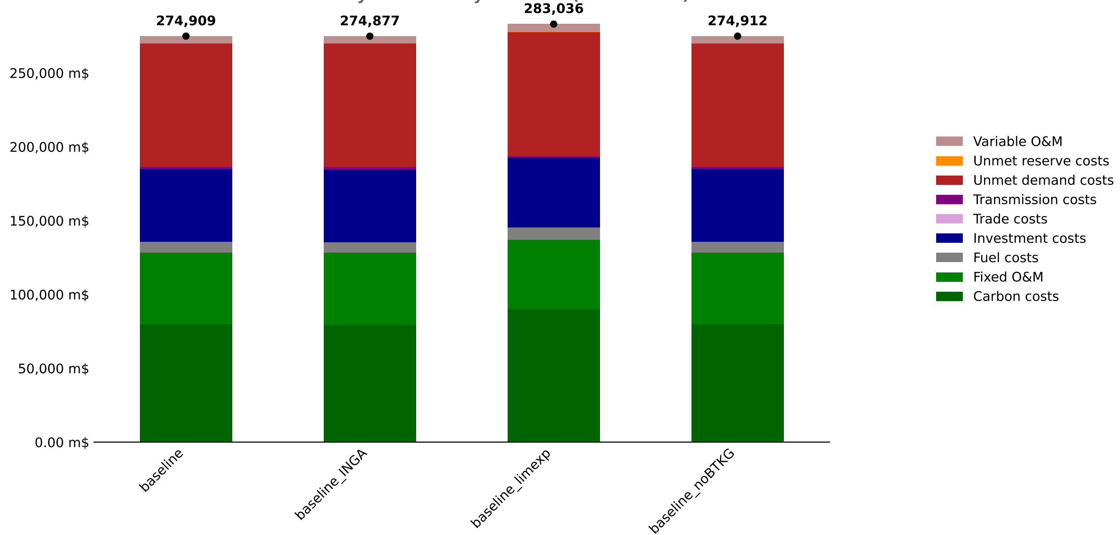
Net Present System Cost by Scenario (million USD)
