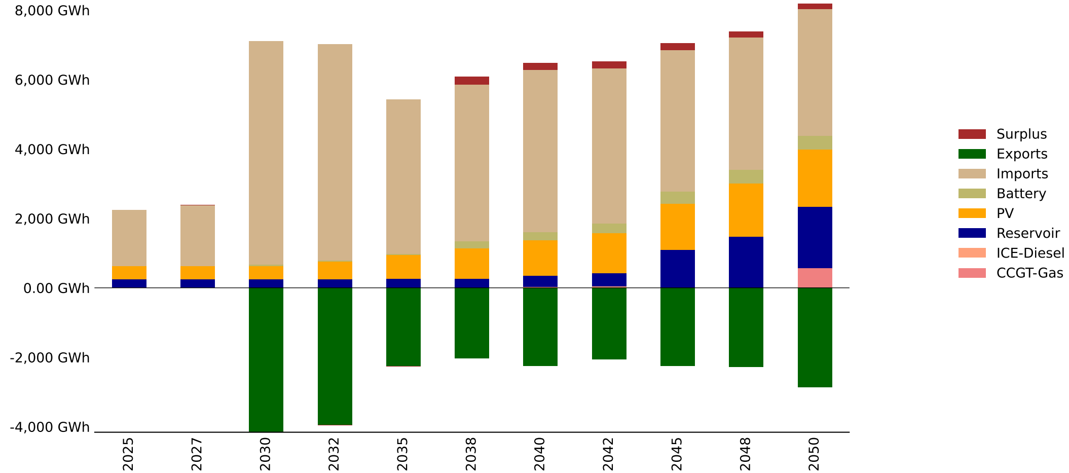
Energy Mix by Fuel - Angola_Central - baseline (GWh)
