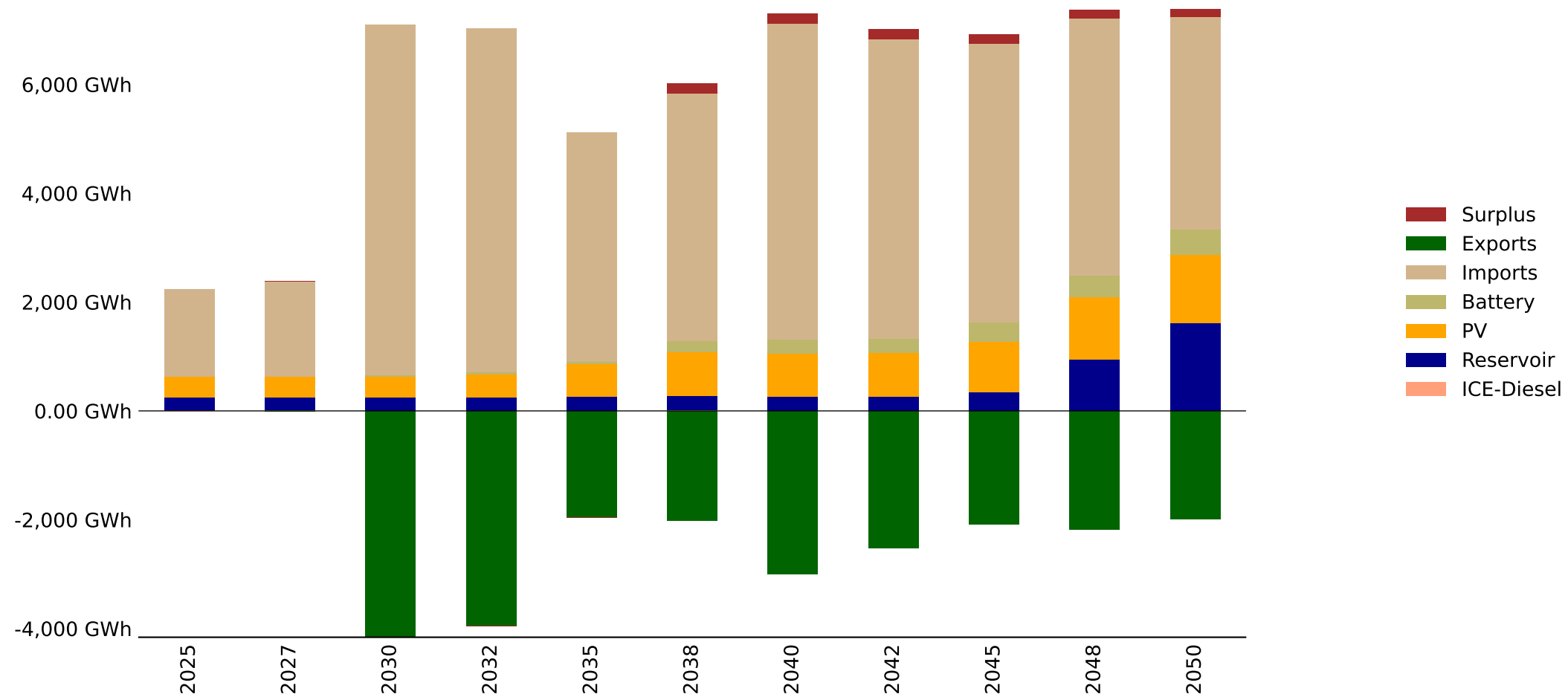
Energy Mix by Fuel - Angola_Central - baseline_INGA (GWh)
