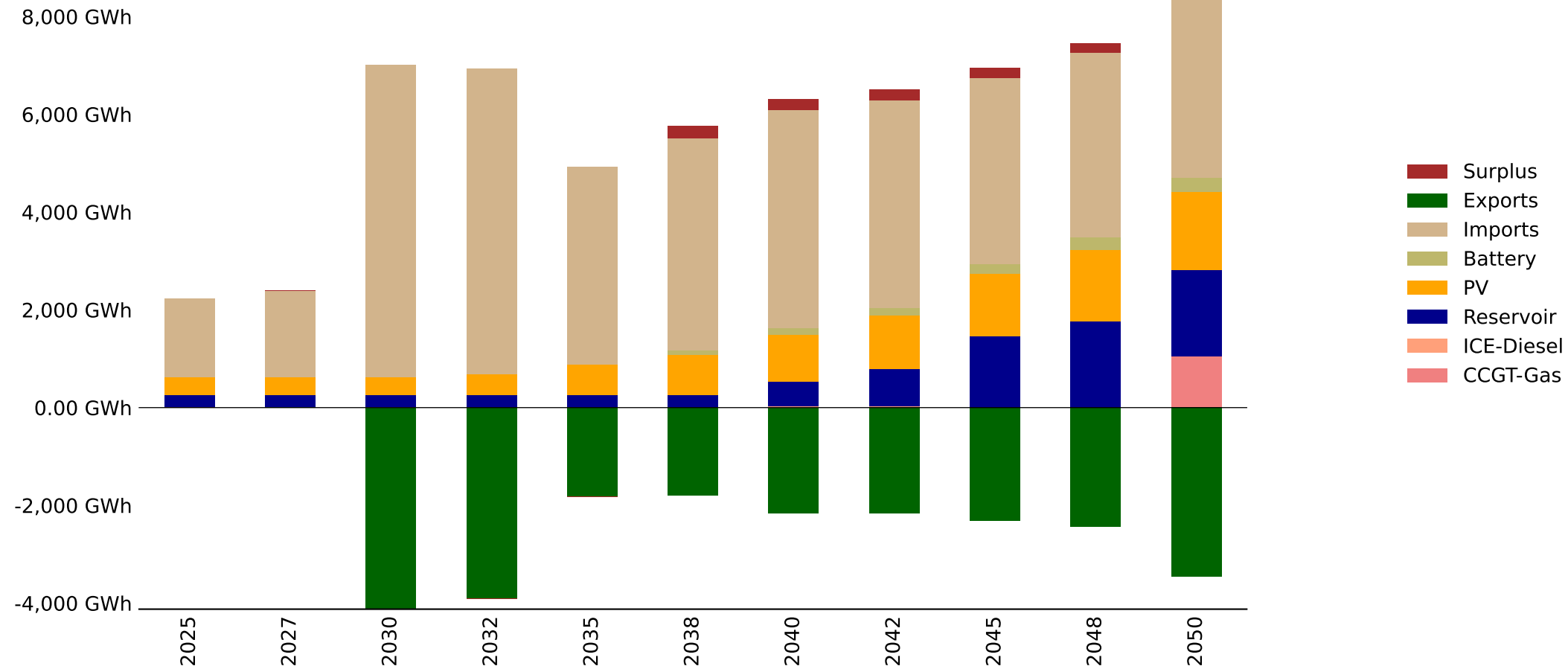
Energy Mix by Fuel - Angola_Central - baseline_limexp (GWh)
