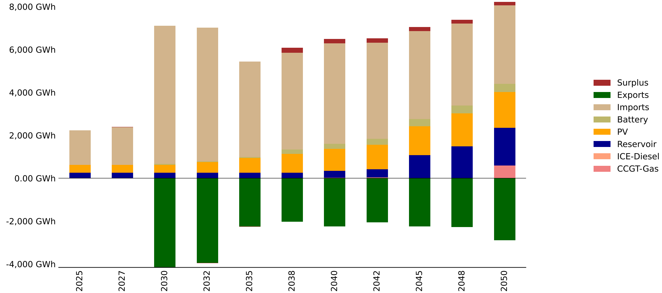
Energy Mix by Fuel - Angola_Central - baseline_noBTKG (GWh)
