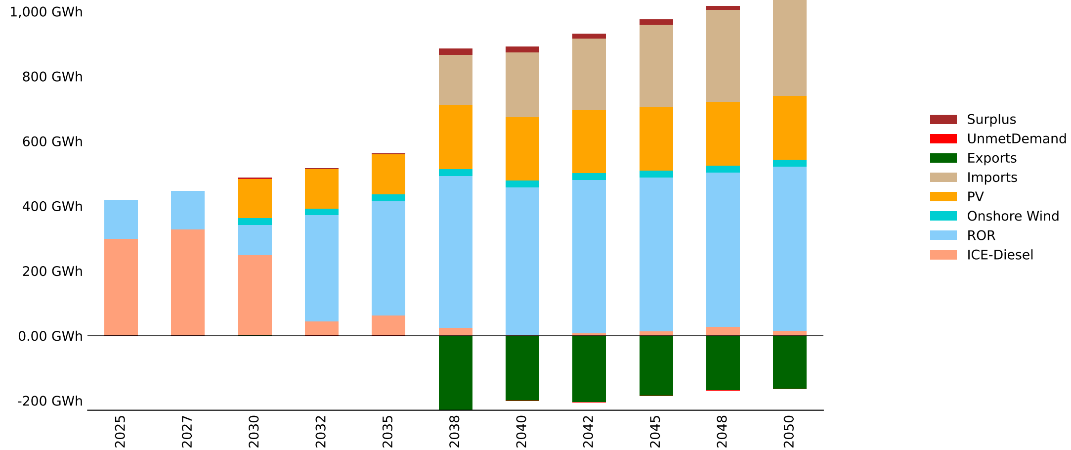
Energy Mix by Fuel - Angola_East - baseline_INGA (GWh)
