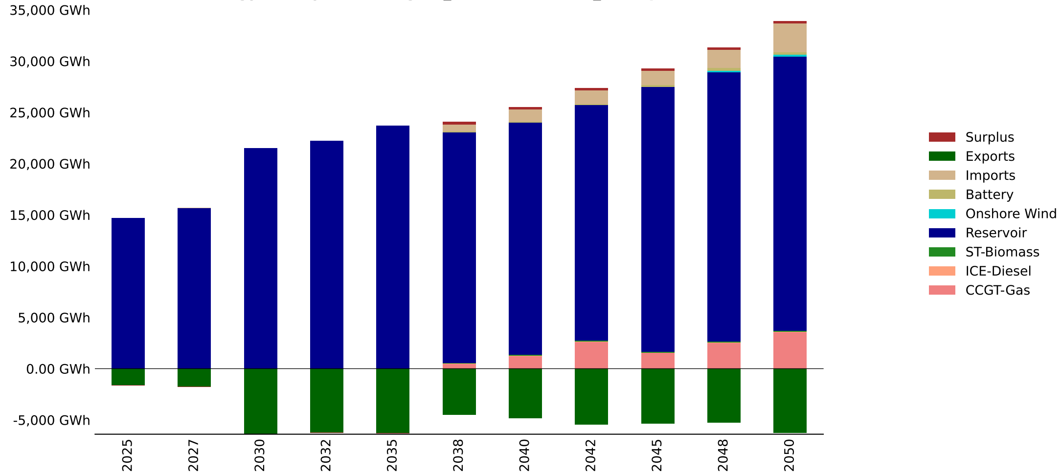
Energy Mix by Fuel - Angola_North - baseline_limexp (GWh)
