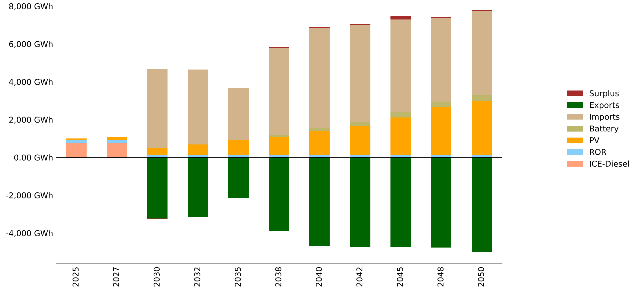
Energy Mix by Fuel - Angola_South - baseline (GWh)
