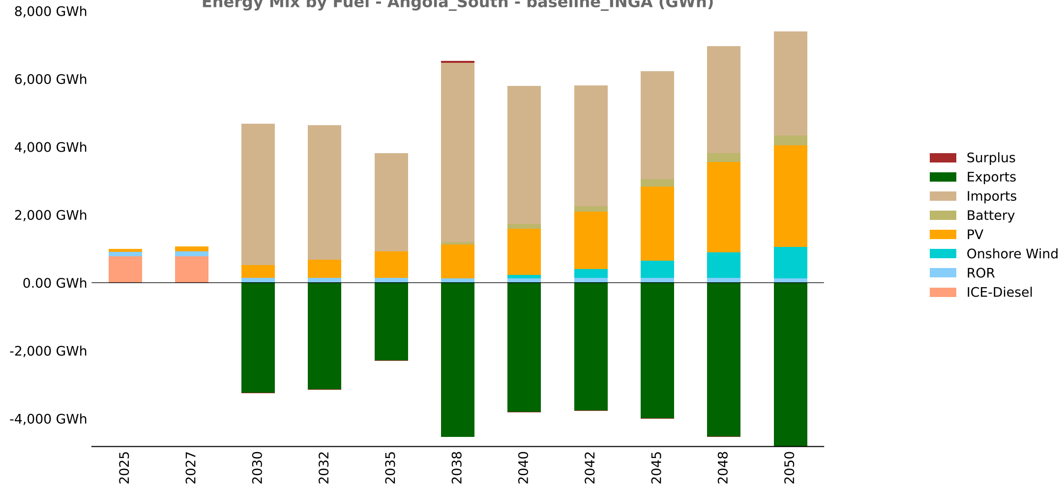
Energy Mix by Fuel - Angola_South - baseline_INGA (GWh)
