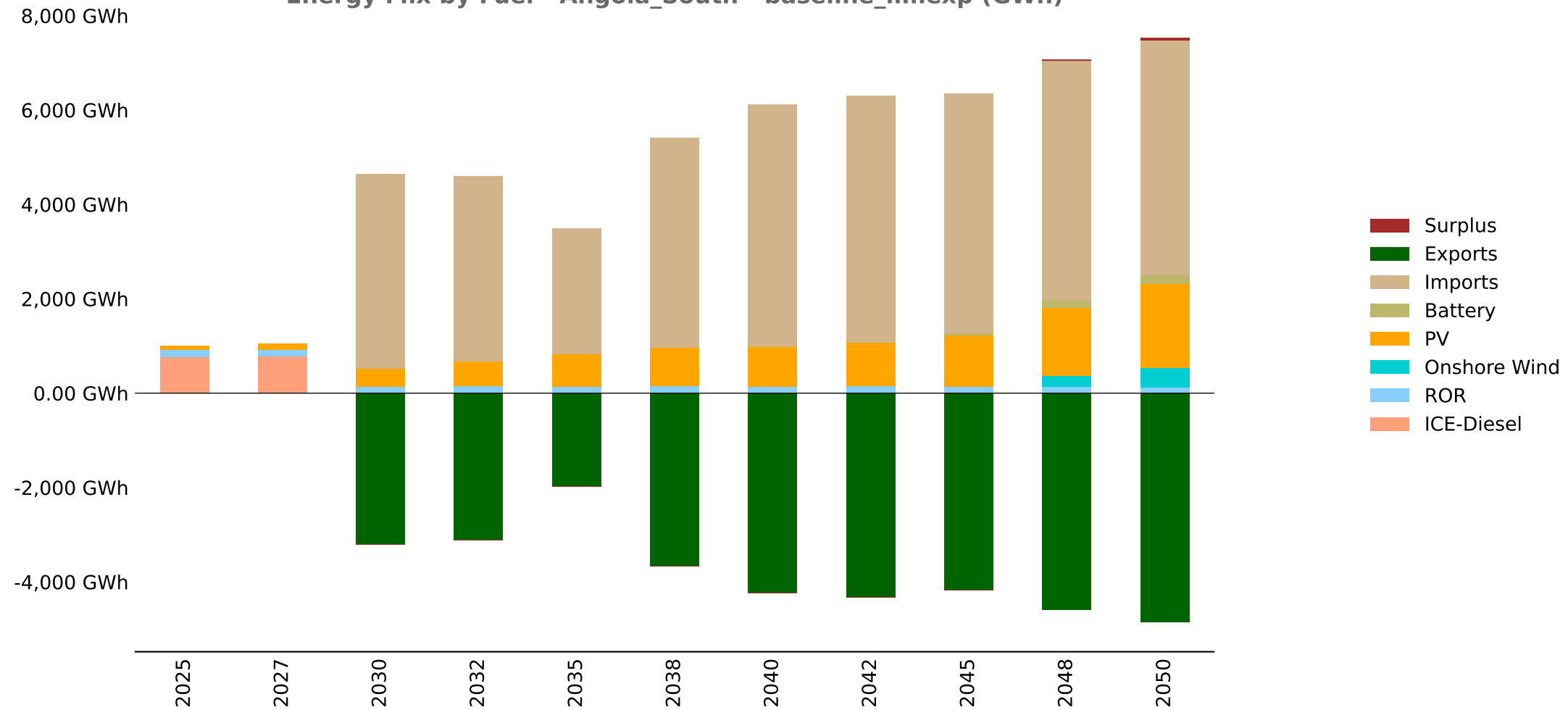
Energy Mix by Fuel - Angola_South - baseline_limexp (GWh)
