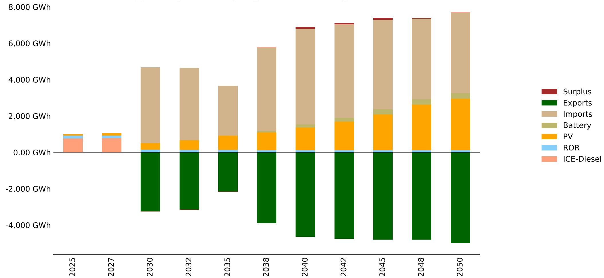
Energy Mix by Fuel - Angola_South - baseline_noBTKG (GWh)
